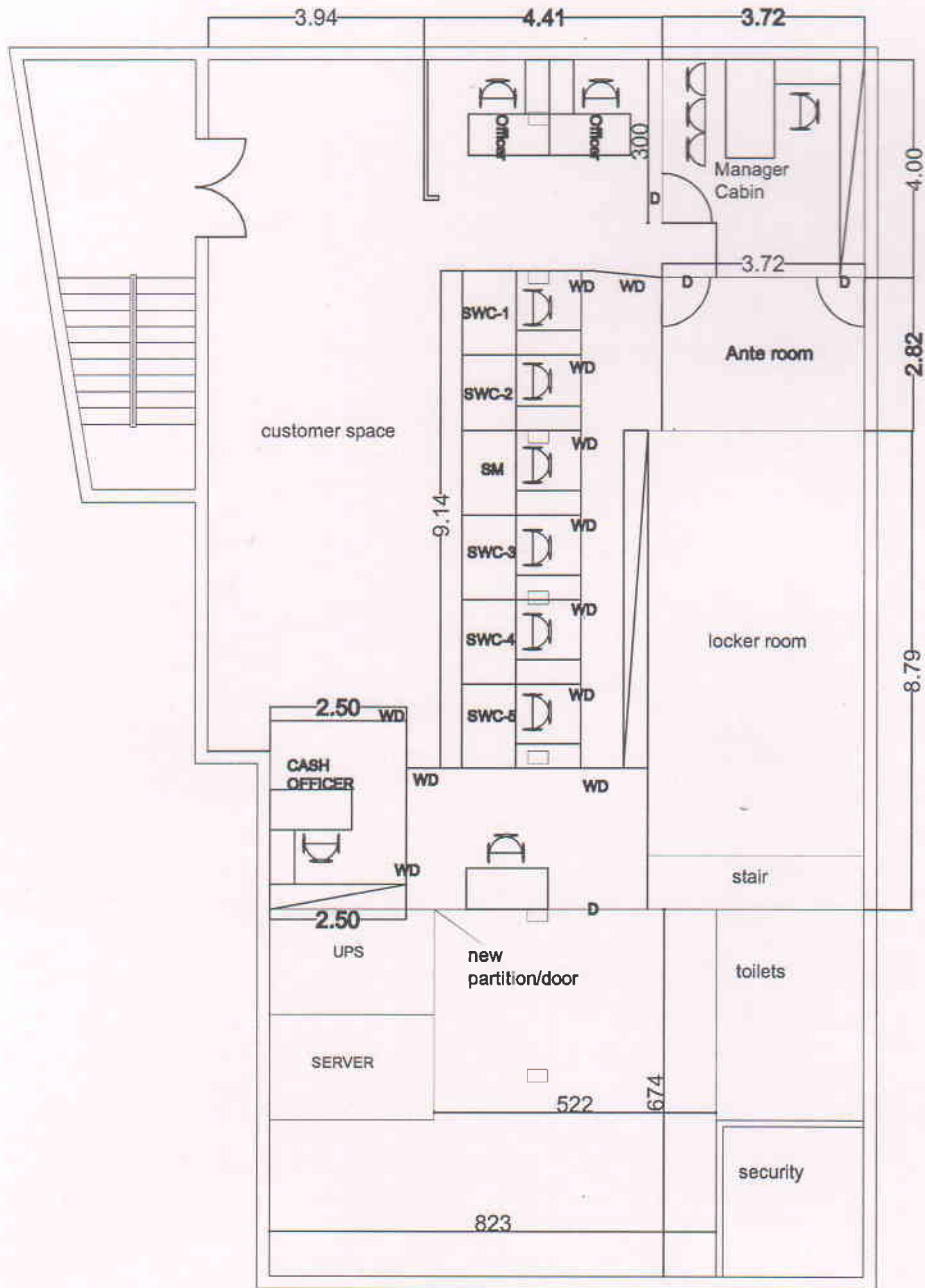
SBI COLLEGE ROAD - KATTAKADA(RENOVATION) First floor -proposed plan- 12.11.2020
